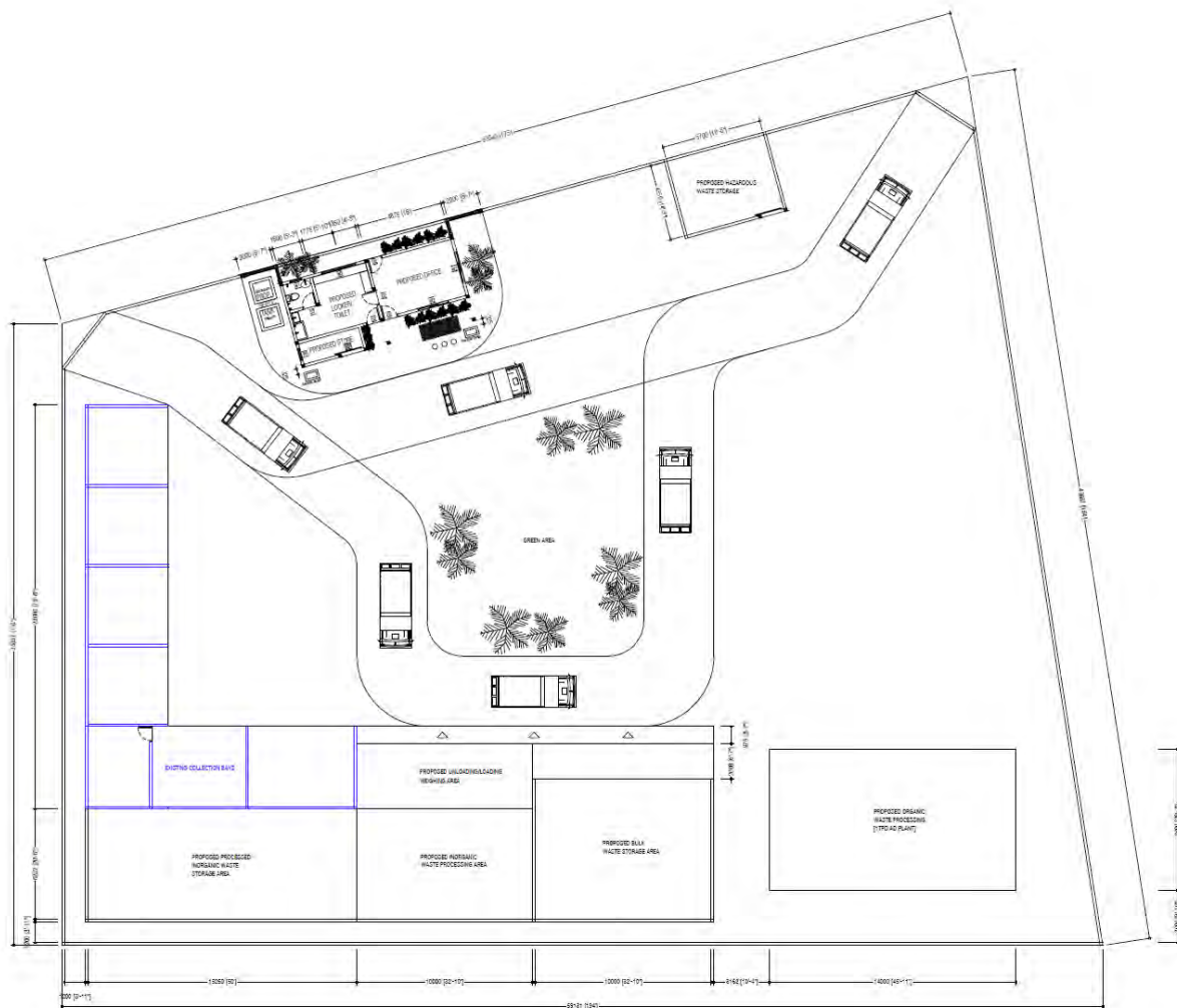
Figure 2. Schematic layout of IWRMC proposed (scaled site plan given in Appendix 6)
