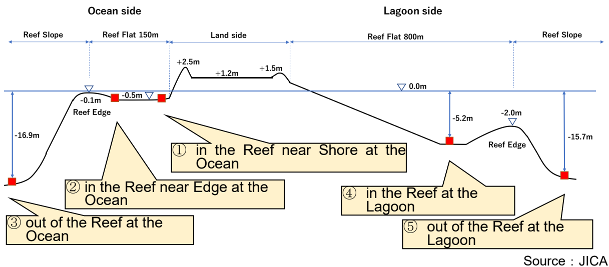
Figure 2.1.15 Location of the Hydraulic Wave Height Meter
