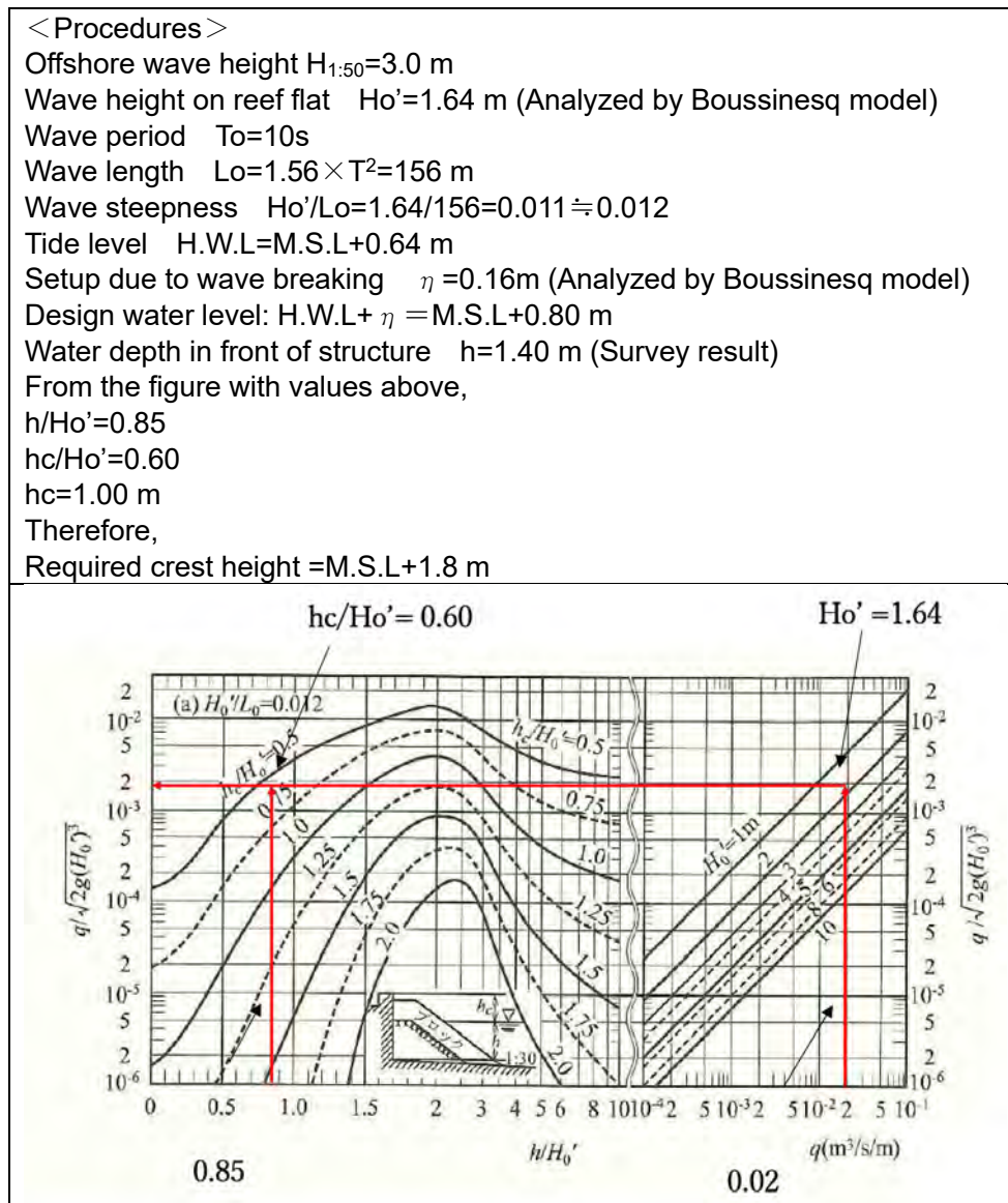
Figure 9.2.5 Calculation of Required Crest Height against H1:50 (Maamendhoo)
