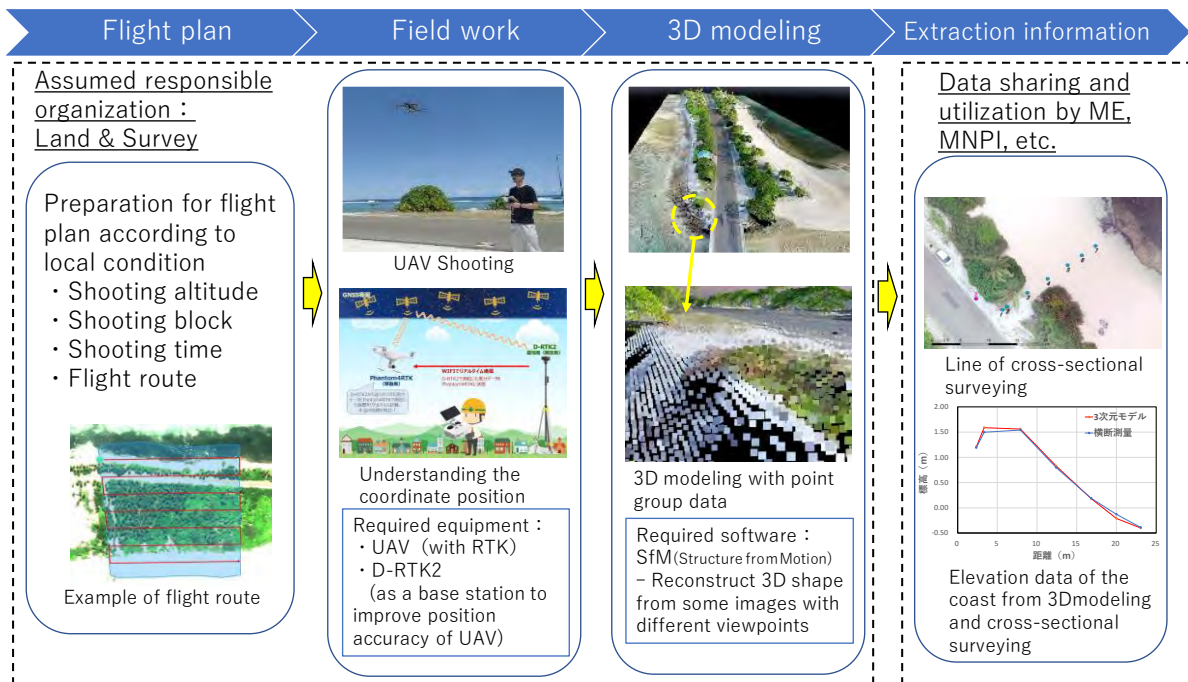
Figure 8.5.3 Image of Monitoring System using UAV Technology
