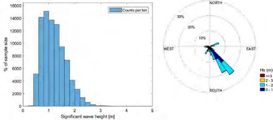
Source: Assessment of extreme and metocean conditions in the Maldives for OTEC applications (2019) 5) Figure 2.1.13 Distribution and Rose for Significant Wave (1979-2008)
