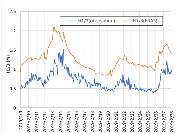
Figure 2.1.11 Time Series Variation of Reanalysis Data (ERA5) and Observation Data of H_{1/3} (Vertical : H_{1/3} (m), Horizontal : Date)
