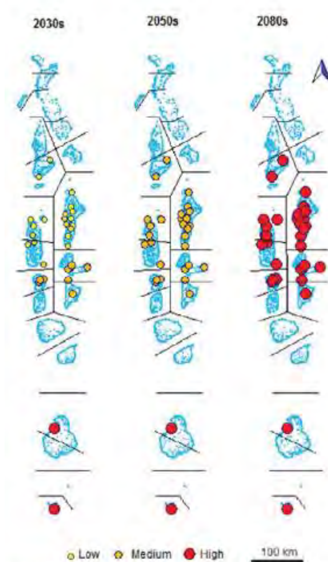
Figure 4.7.3 Projected impacts of coral bleaching
