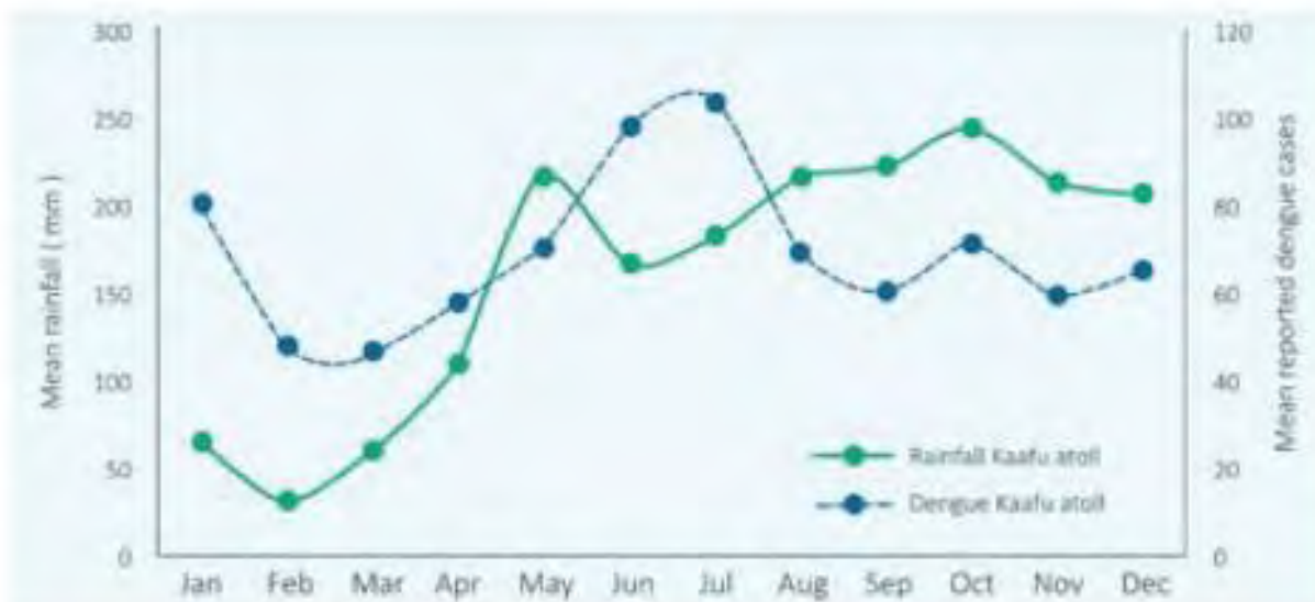
Figure 4.5.2 Reported dengue cases and long term mean rainfall (2005- 2013)
