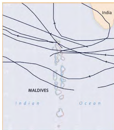
Figure 3.3.1 Cyclones Pathways (1877-2004)
