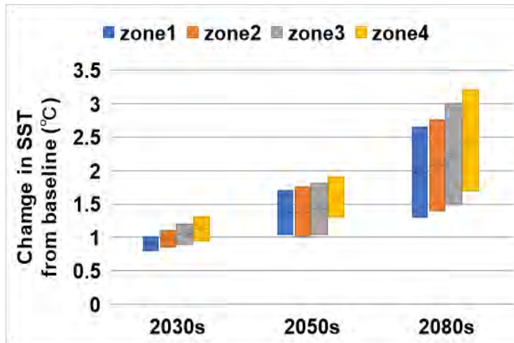
Figure 3.2.8 Estimated Sea Surface Temperature Rise
