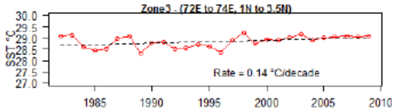
Figure 6.4.7 Variation of annual mean sea surface temperature fluctuation for zone 3 in Maldives (1982 to 2009)
