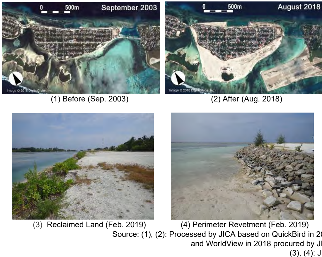
Figure 2.7.3 Feydhoo Reclamation Project
