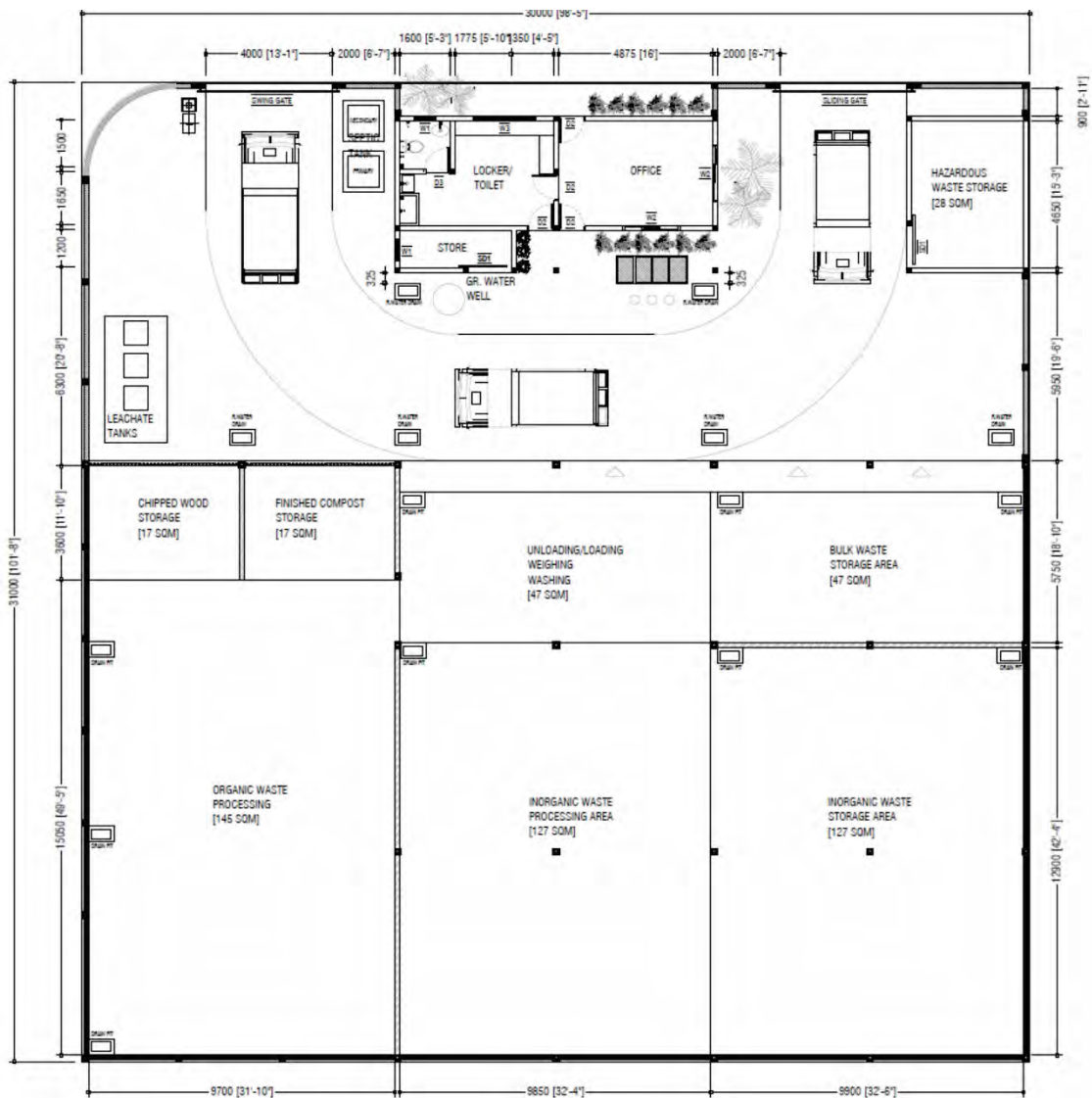
Figure 2. Schematic layout of proposed IWRMC (scaled site plan given in Appendix 4)
