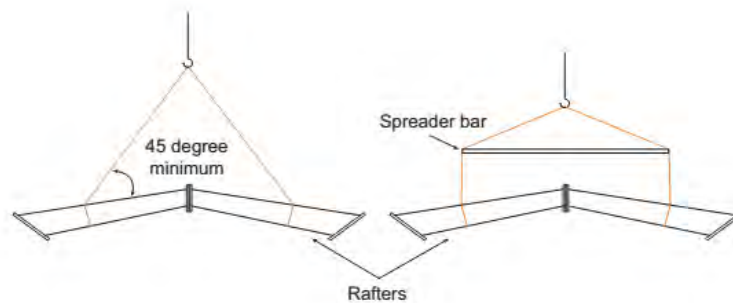
FIGURE 3 HOISTING CABLES
