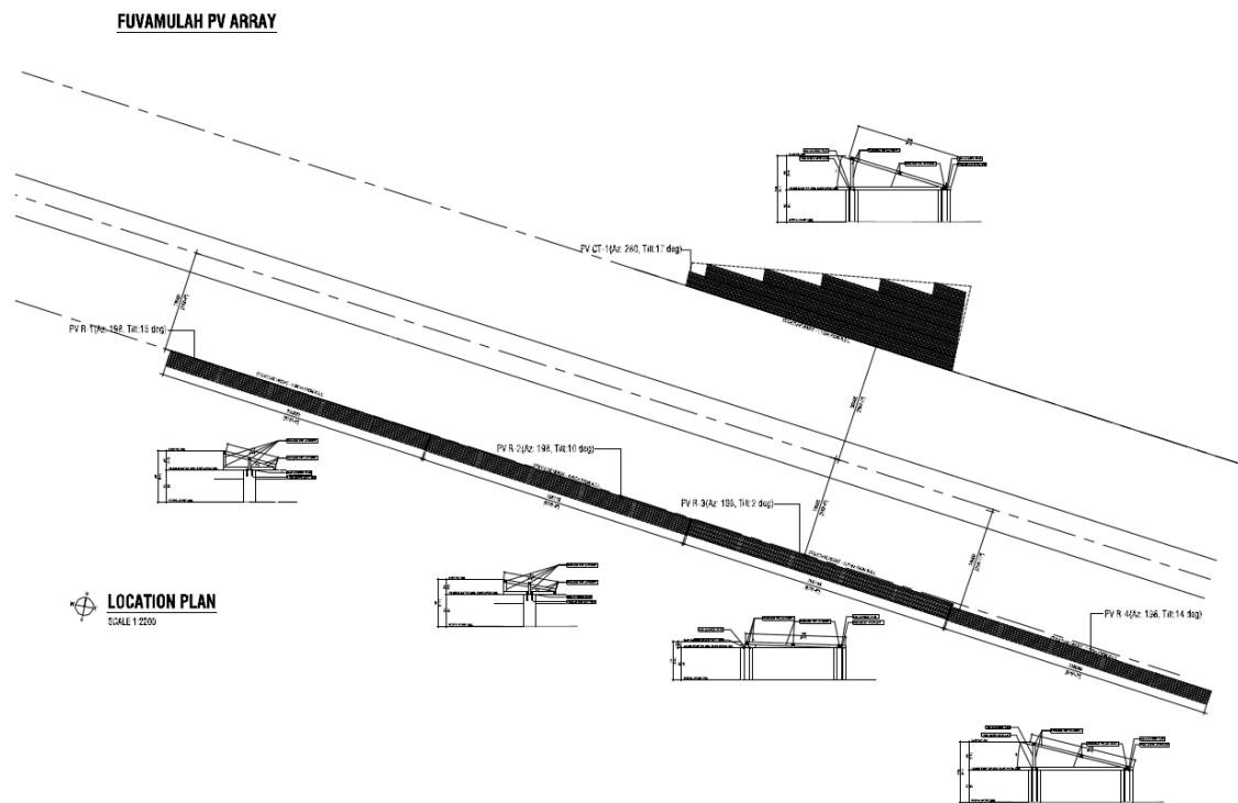
FIGURE 2 FUVAHMULAH AIRPORT PV LAYOUT
