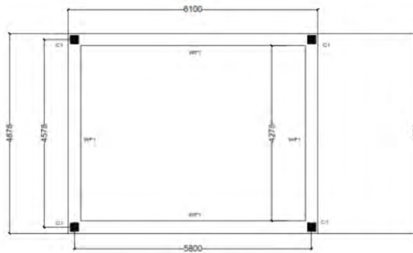
Foundation Details
