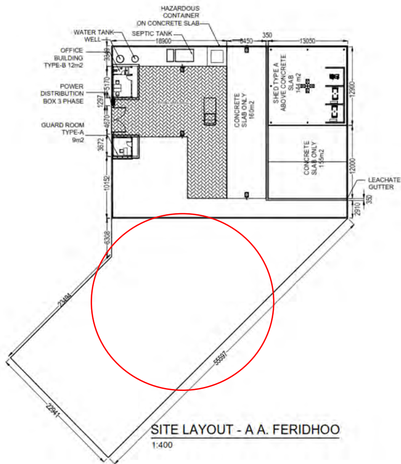
Figure 7: Future expansion area
