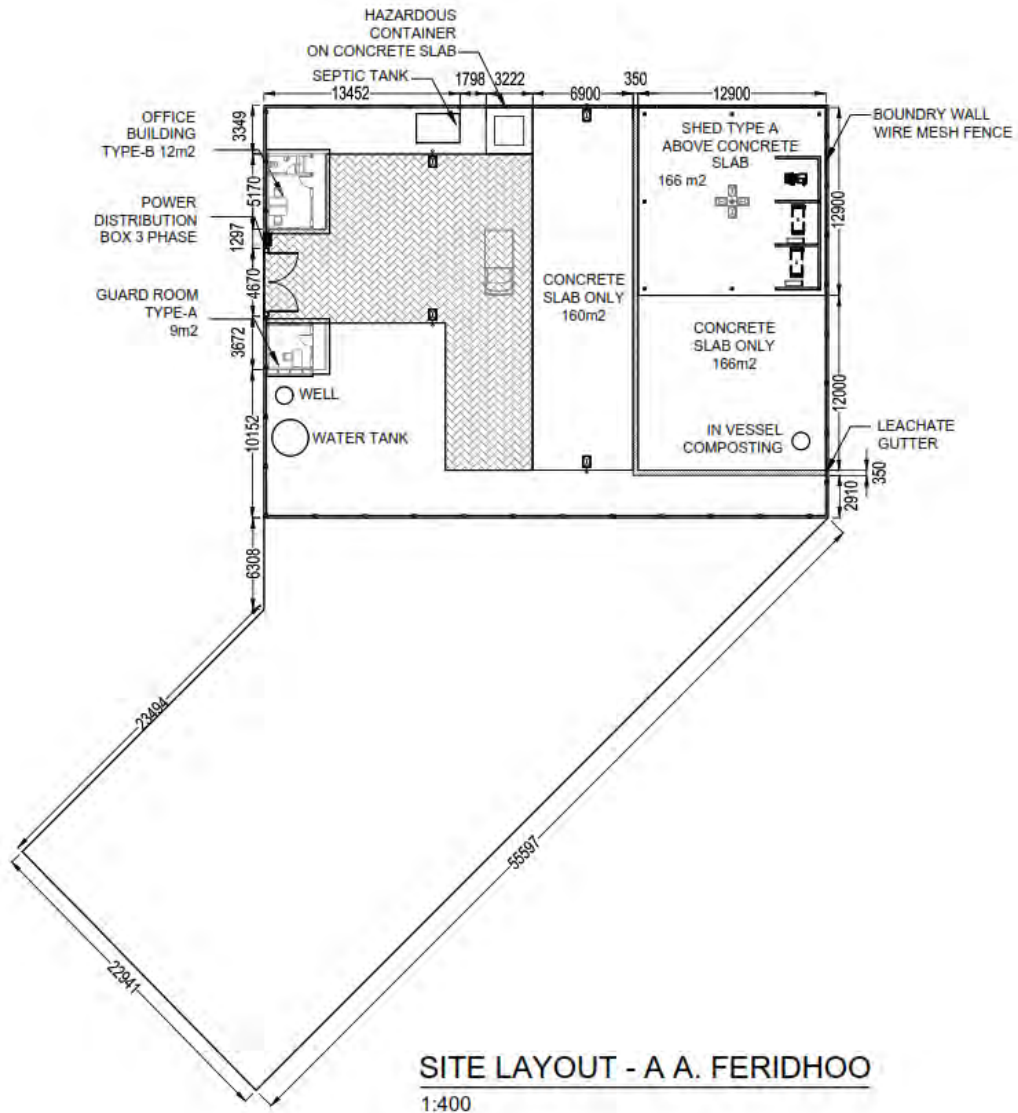
Figure 6: ISWMC concept of Feridhoo island
