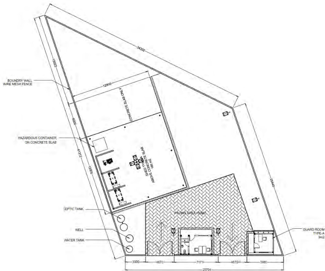
Figure 6: ISWMC concept of Keyodhoo island
