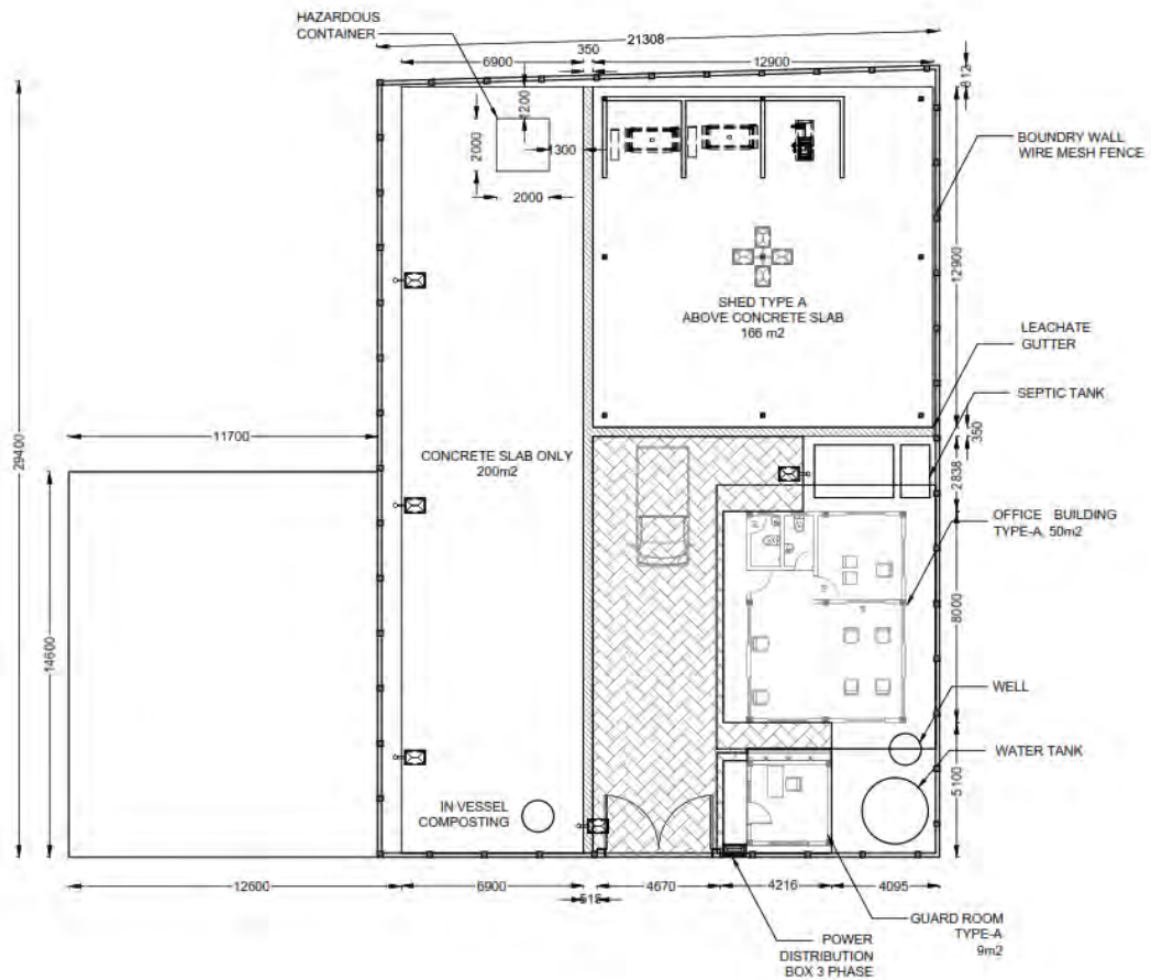
Figure 6: ISWMC concept of Mahibadhoo island
