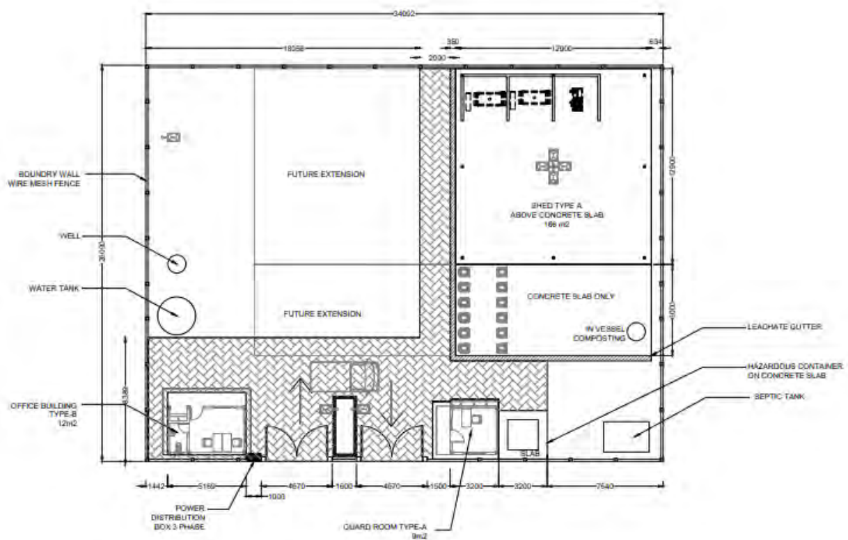
Figure 8: ISWMC concept of Guraidhoo island
