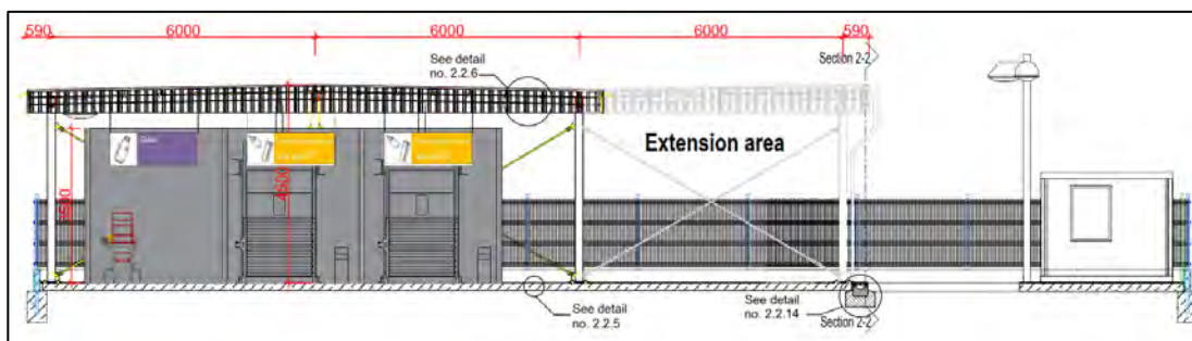
Figure 9: Cross section view of the ISWMC proposed in Guraidhoo
