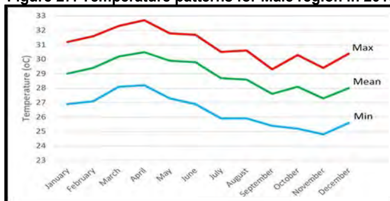
Figure 27: Temperature patterns for Malé region in 2016
