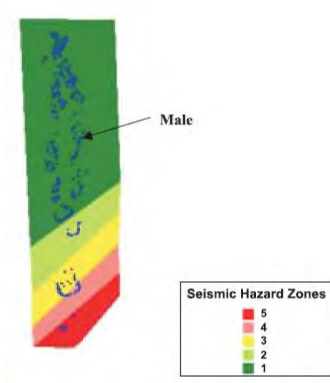
FIGURE 12 MALDIVES SEISMIC HARZARD ZONES (SOURCE: UNDP, 2006)
