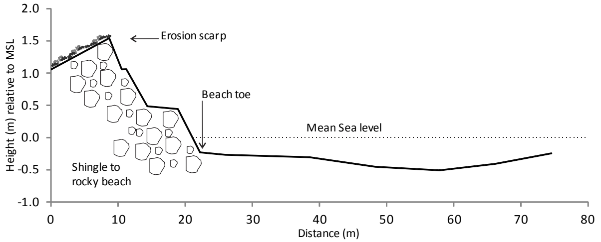
FIGURE 21 BEACH PROFILE 3
