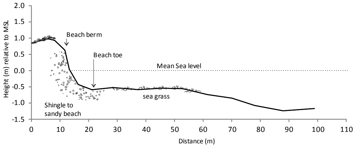
FIGURE 20 BEACH PROFILE 2
