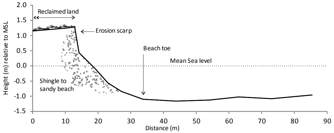
FIGURE 25 BEACH PROFILE 7
