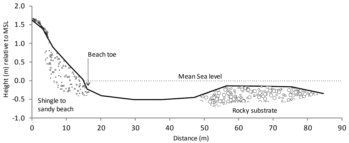
FIGURE 22 BEACH PROFILE 4
