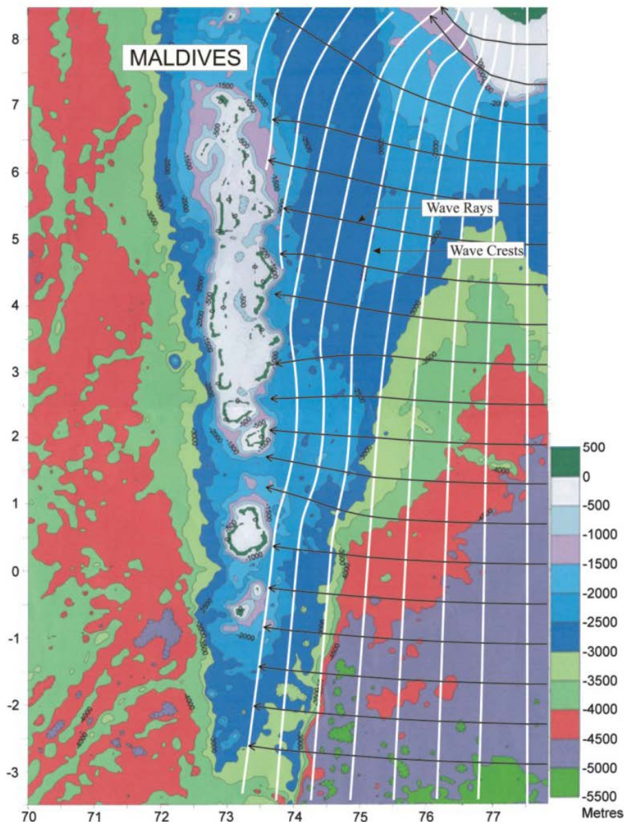
FIGURE 10 INDIAN OCEAN BATHYMETRY AND TSUNAMI PROPAGATION MODEL (SOURCE: ALI, 2005)
