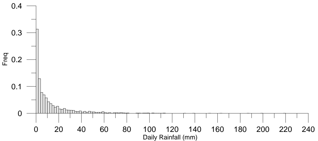
FIGURE 7 FREQUENCY OF THE DAILY RAINFALL
