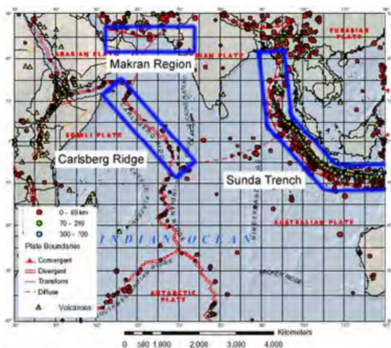
FIGURE 9 TSUNAMI SOURCE AND SIGNIFICANT EARTHQUAKE IN THE INDIAN OCEAN (SOURCE: USGS, 2003)
