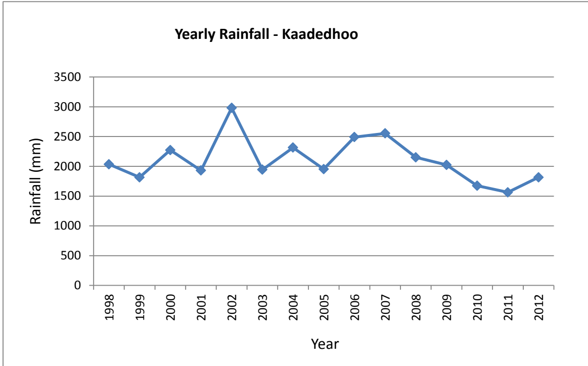
FIGURE 6 ANNUAL RAINFALL FOR THE 15-YEAR PERIOD BETWEEN 1998 AND 2012 (MMS , 2013)
