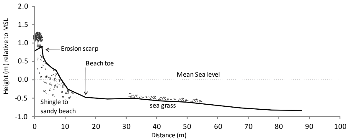
FIGURE 24 BEACH PROFILE 6
