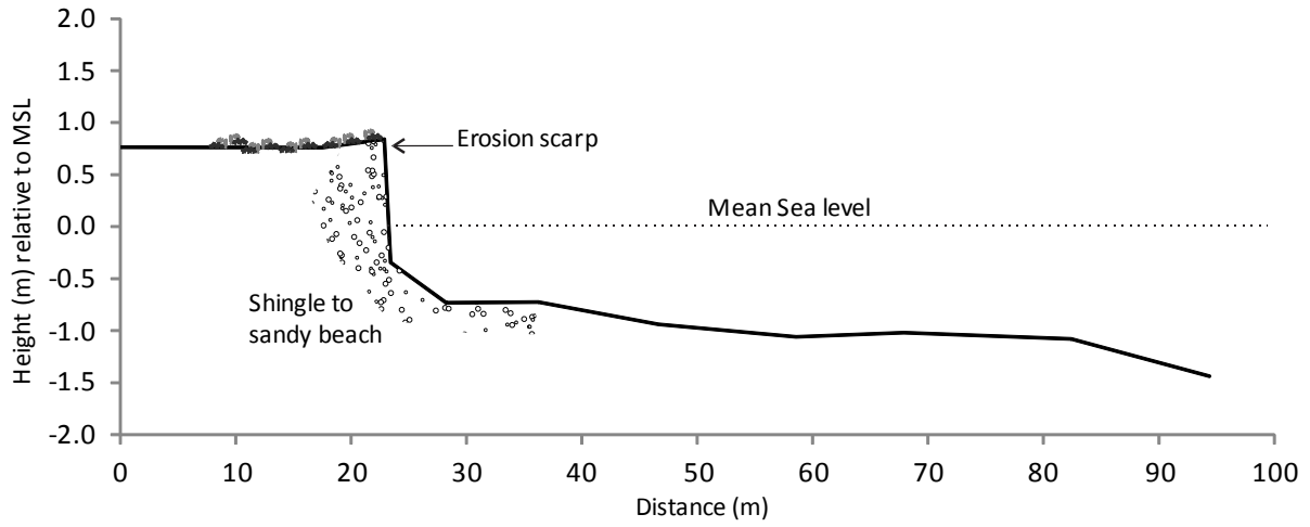
FIGURE 19 BEACH PROFILE 1
