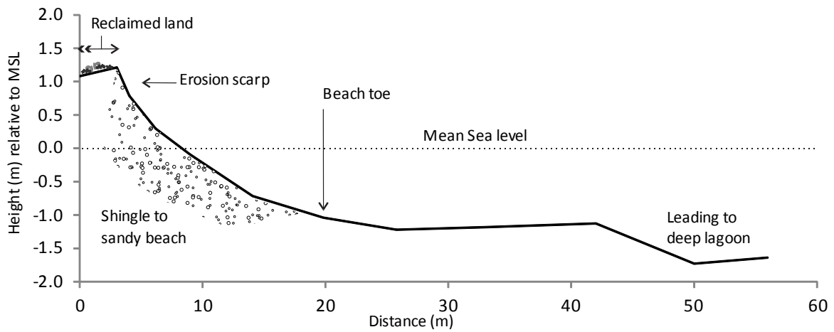
FIGURE 26 BEACH PROFILE 8
