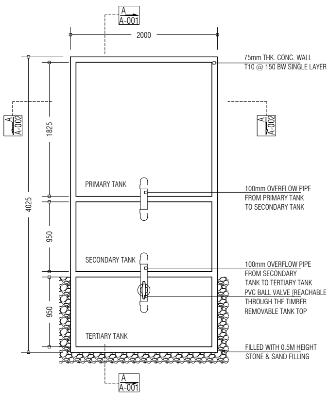
PLAN
