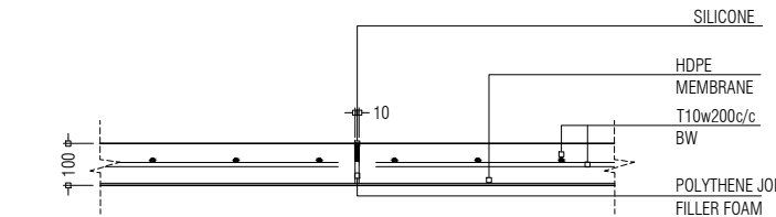
COMPOST BED SLAB DETAIL 1:20
