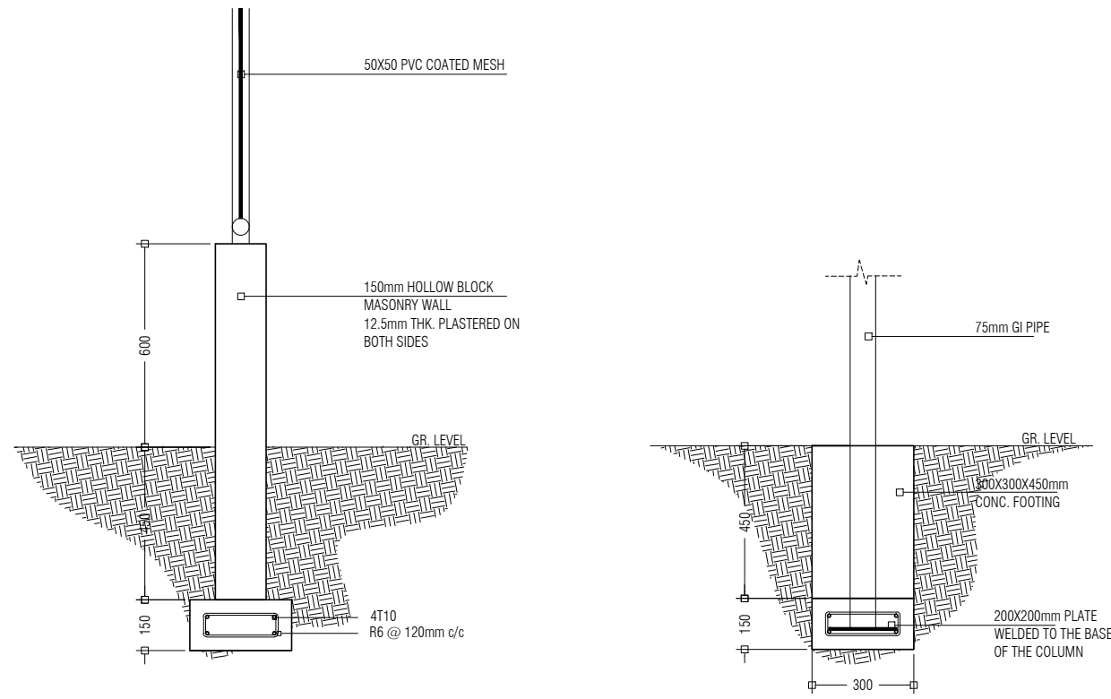
PERIMETER FENCE WALL FOUNDATION DETAIL
