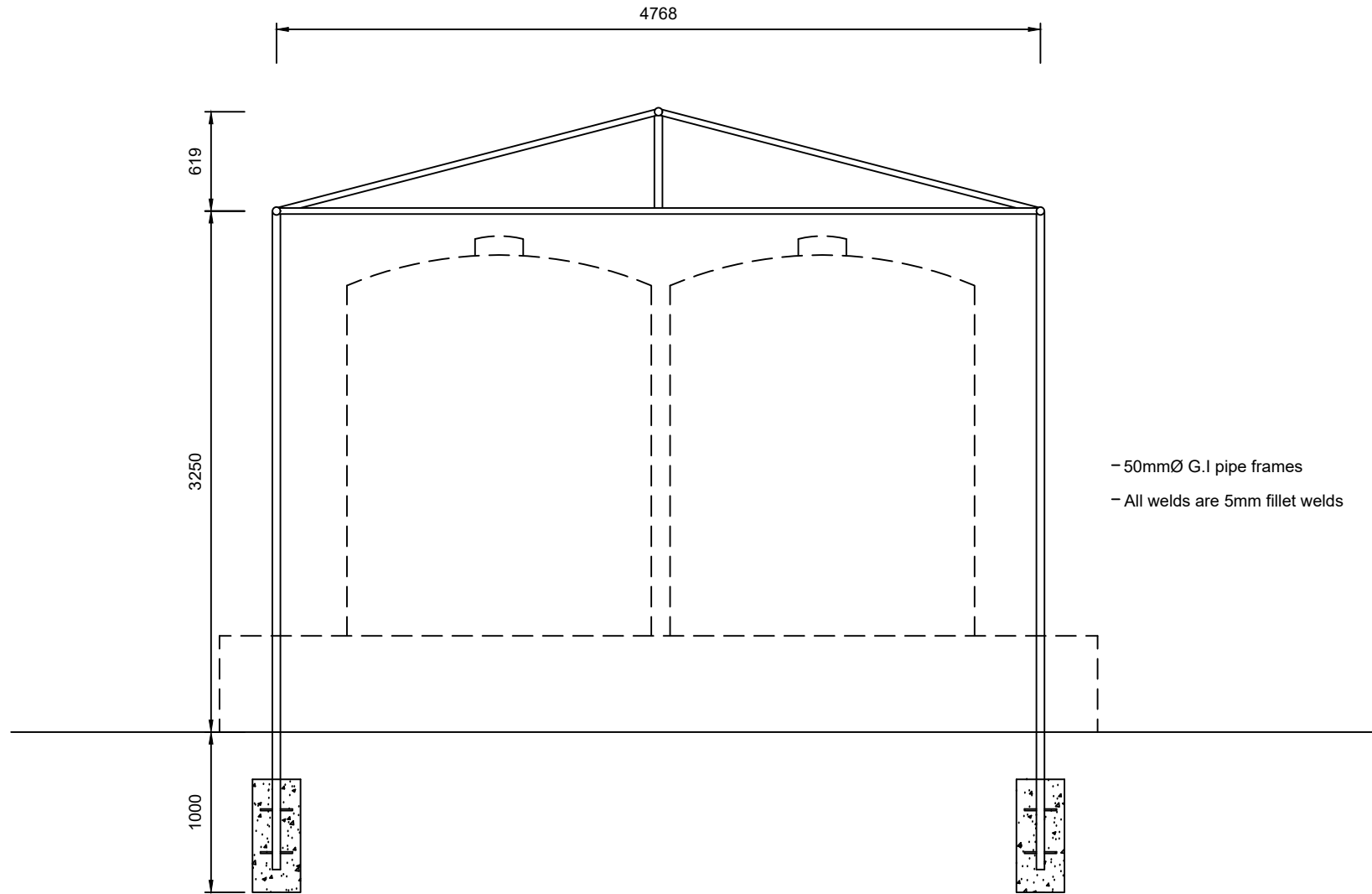
ROOF SUPPORTING FRAME DETAIL MASJIDUL SALAAH
