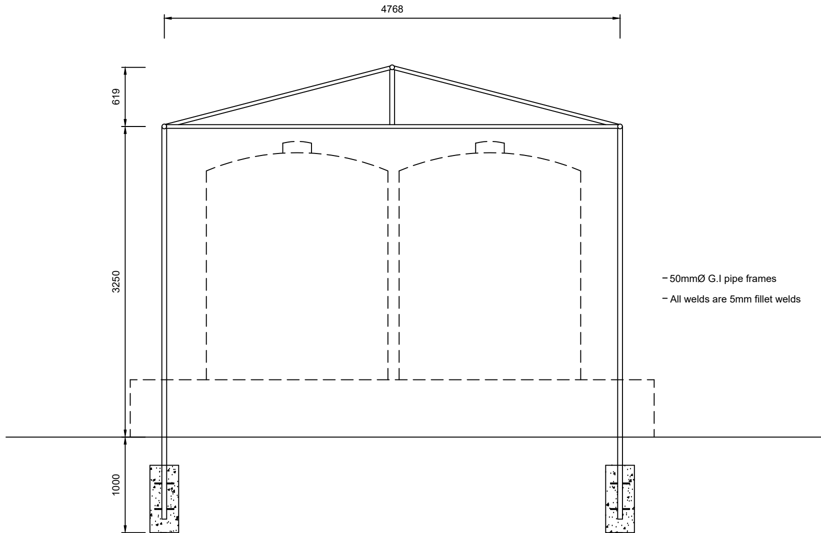
ROOF SUPPORTING FRAME DETAIL PRESCHOOL
