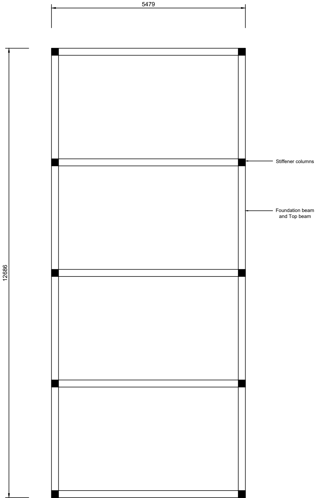
FOUNDATION PLAN MASJIDUL IBRAHIM
