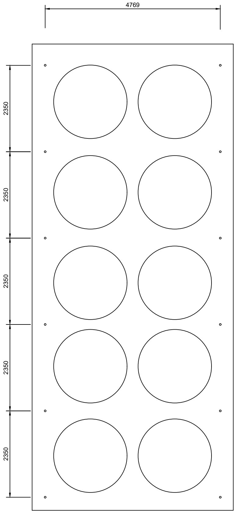
ROOF SUPPORTING PIPE ARRANGEMENT - PLAN MASJIDUL IBRAHIM
