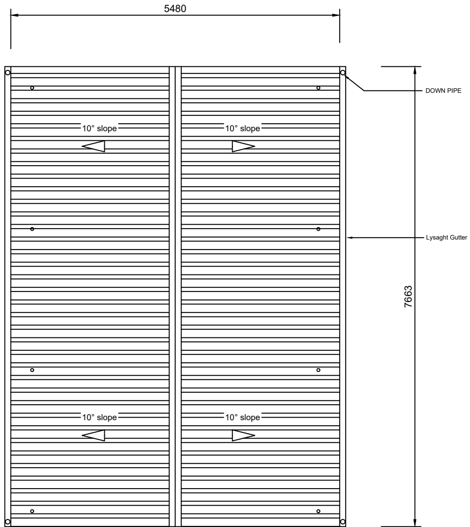
ROOF PLAN OVER WATER TANKS MASJIDUL SALAAH
