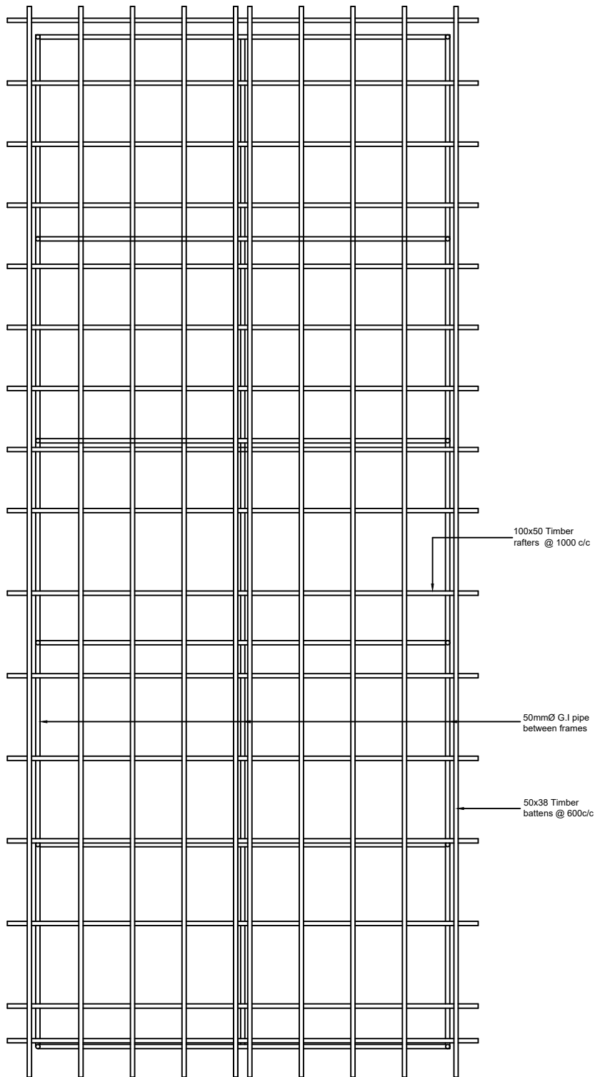
ROOF FRAMING PLAN MASJIDUL IBRAHIM
