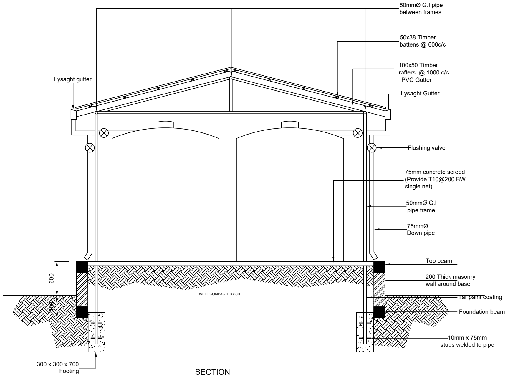
SECTION MASJIDUL SALAAH
