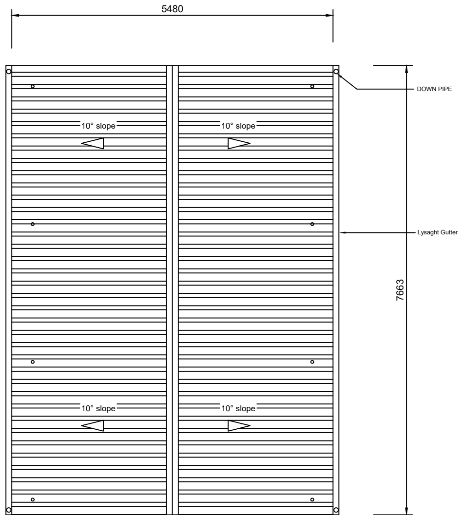
ROOF PLAN OVER WATER TANKS PRESCHOOL
