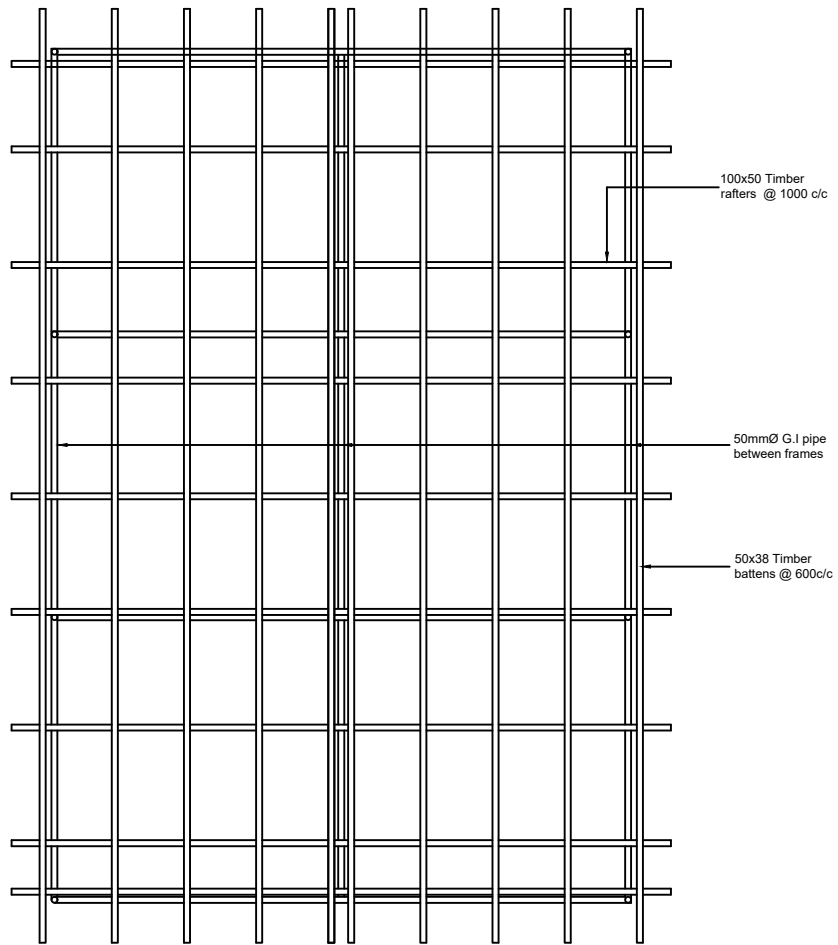
ROOF FRAMING PLAN PRESCHOOL
