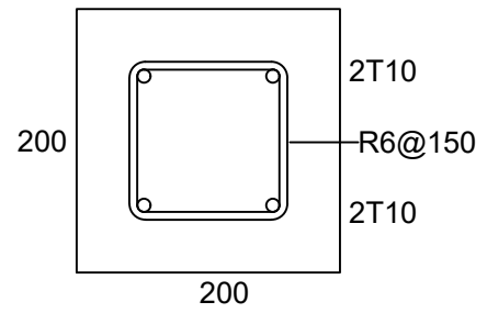
FOUNDATION BEAM
