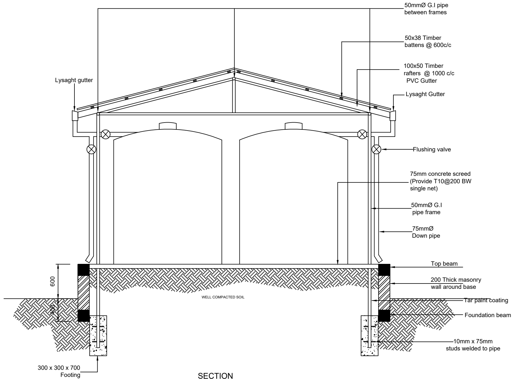
SECTION PRESCHOOL
