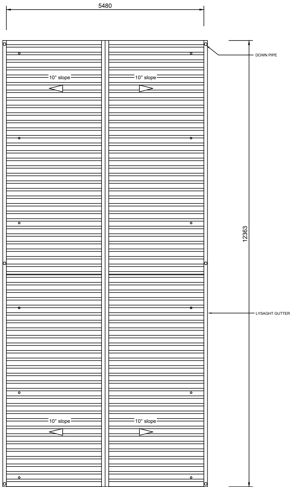
ROOF PLAN OVER WATER TANKS MASJIDUL IBRAHIM
