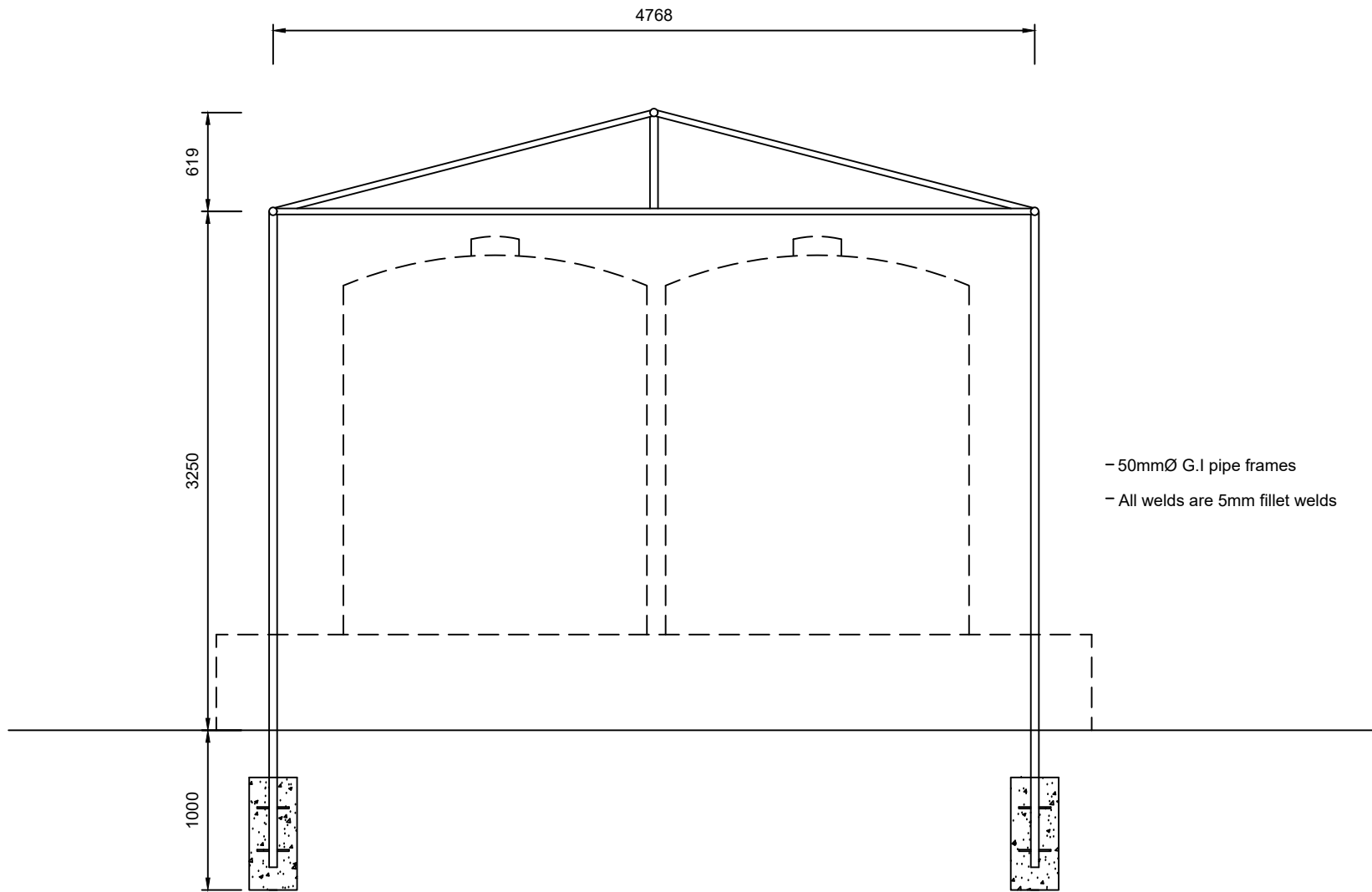
ROOF SUPPORTING FRAME DETAIL MASJIDUL IBRAHIM
