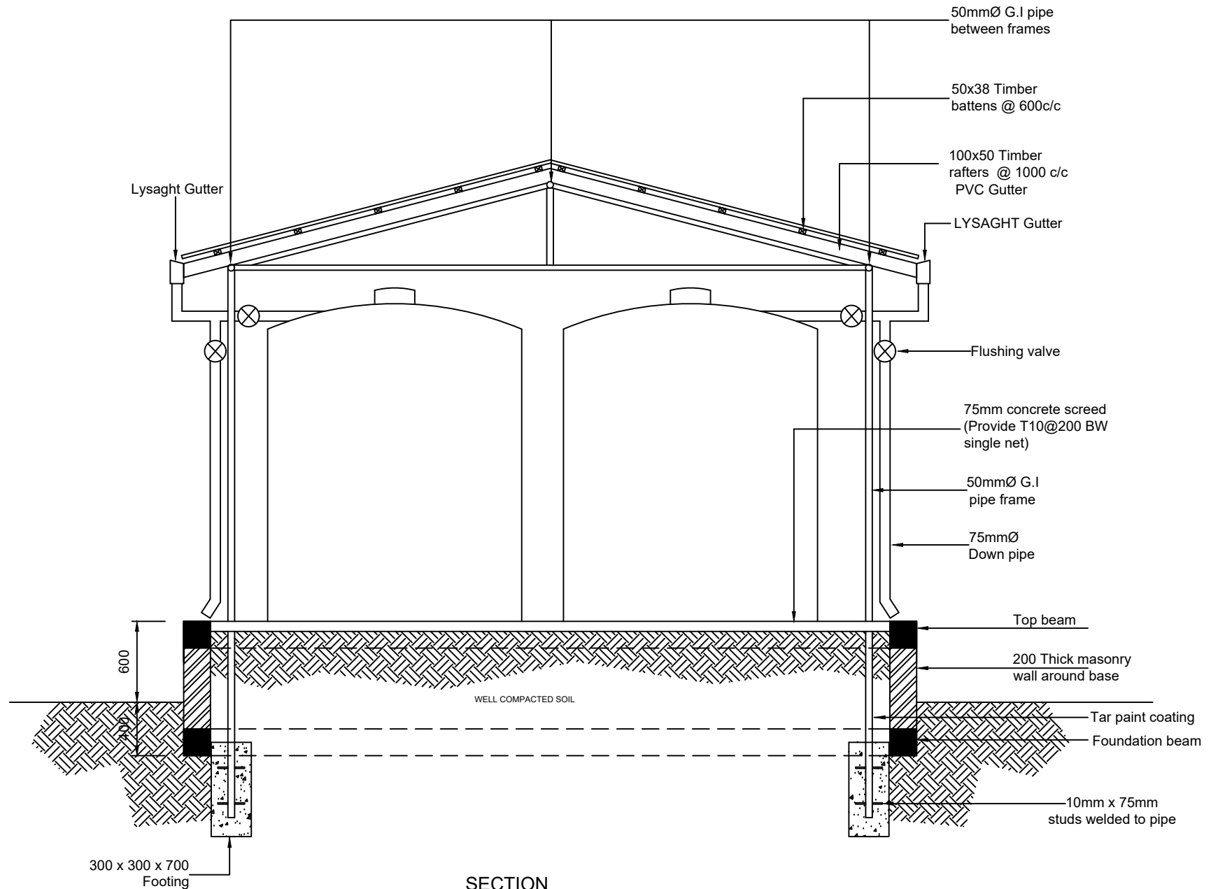
SECTION MASJIDUL IBRAHIM
