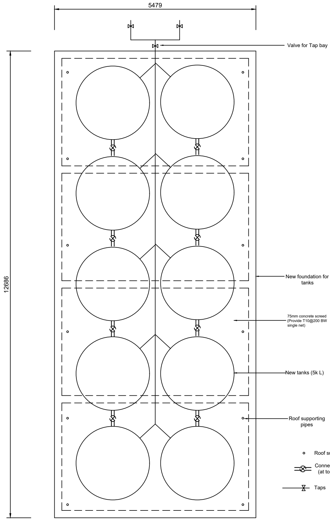
WATER TANK ARRANGEMENT - PLAN MASJIDUL IBRAHIM
