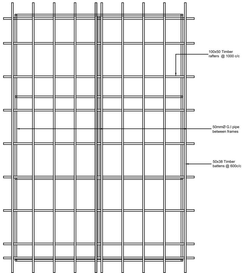
ROOF FRAMING PLAN MASJIDUL SALAAH
