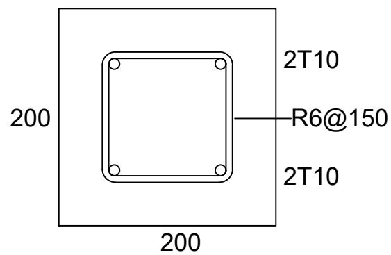
FOUNDATION BEAM
