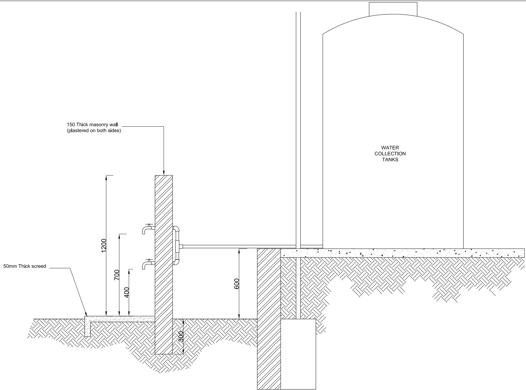
WATER DISTRIBUTION TAPPING STATION SECTION
