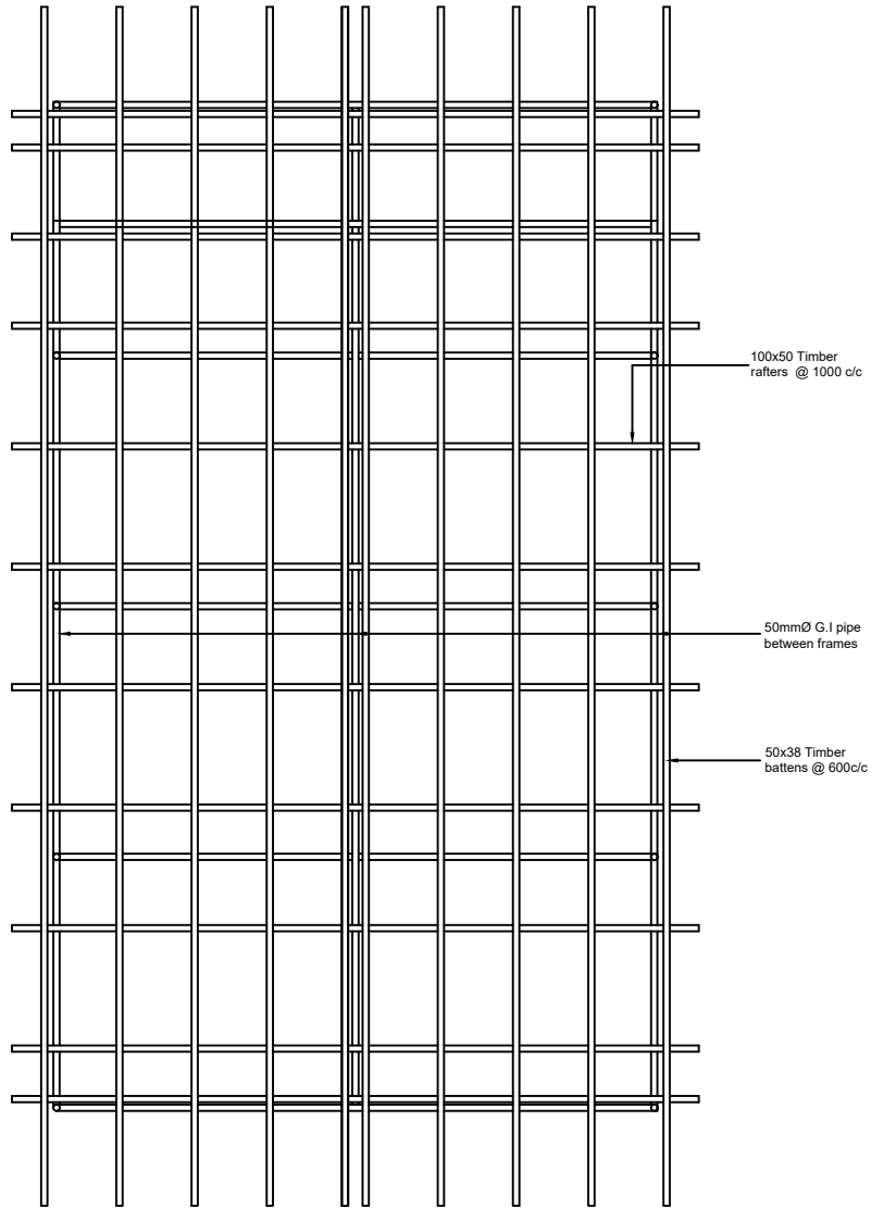
ROOF FRAMING PLAN COUNCIL SITE
