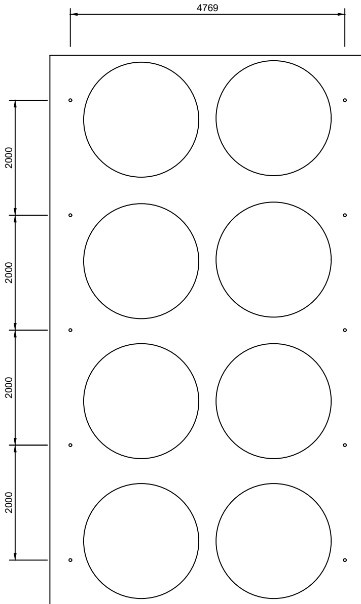
ROOF SUPPORTING PIPE ARRANGEMENT - PLAN COUNCIL SITE
