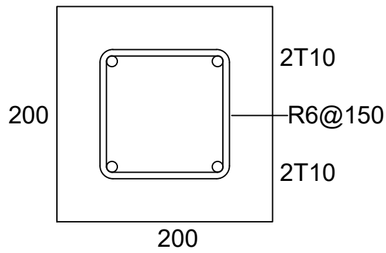
TOP BEAM
