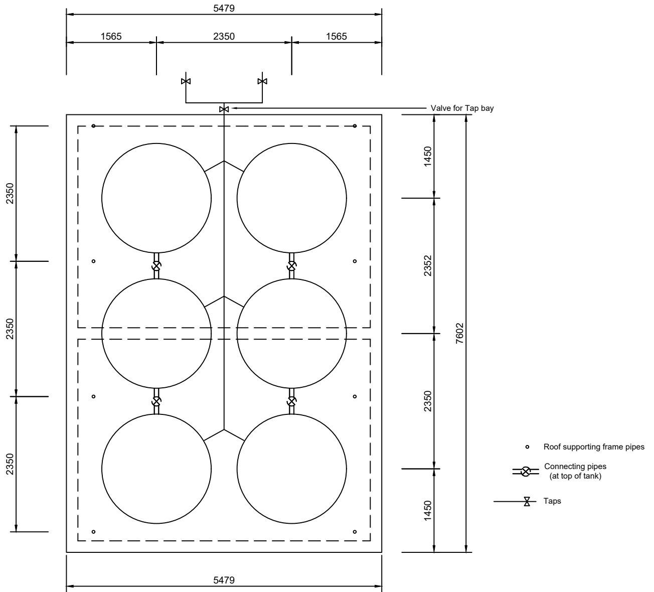
WATER TANK ARRANGEMENT - PLAN STAGE SITE
