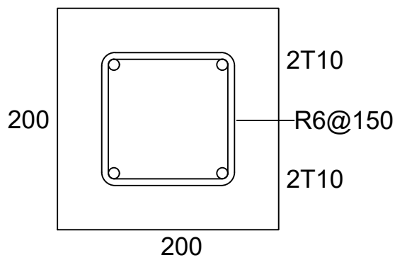
TOP BEAM
