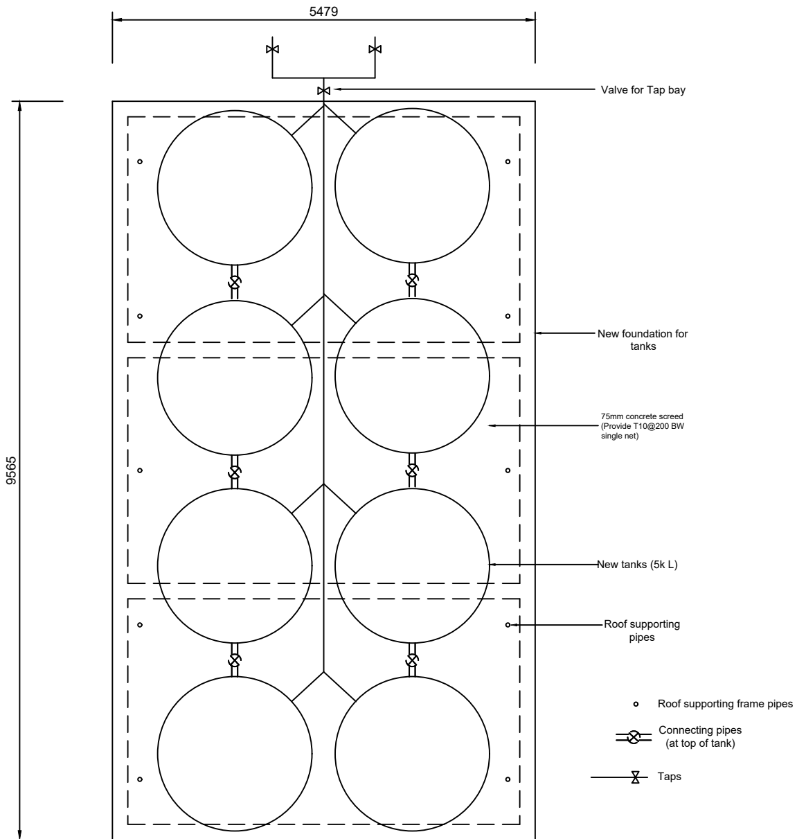
WATER TANK ARRANGEMENT - PLAN COUNCIL SITE
