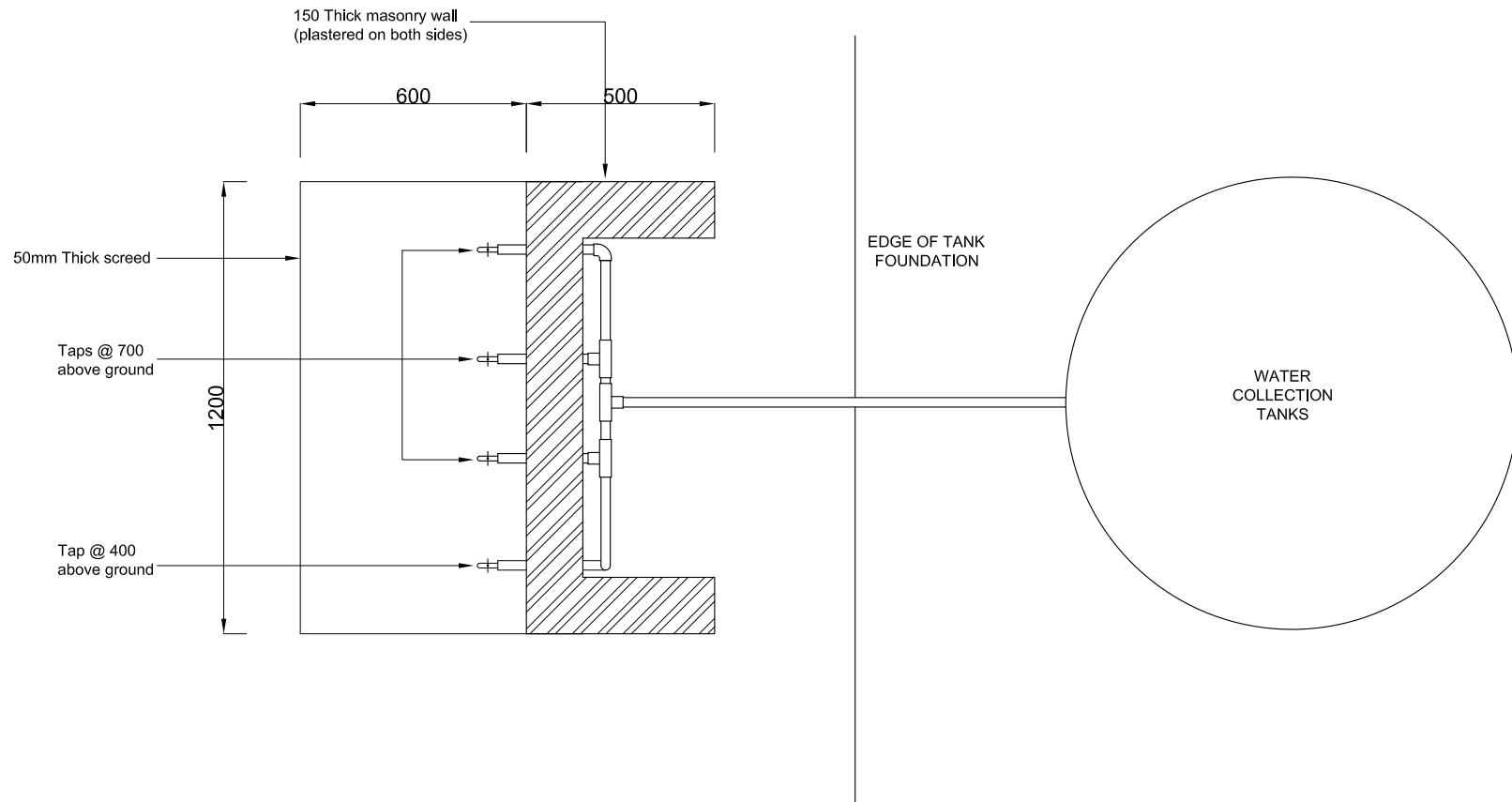
WATER DISTRIBUTION TAPPING STATION PLAN
