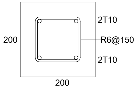
FOUNDATION BEAM
