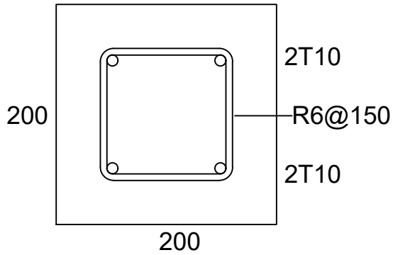
TOP BEAM
