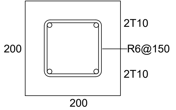
FOUNDATION BEAM
