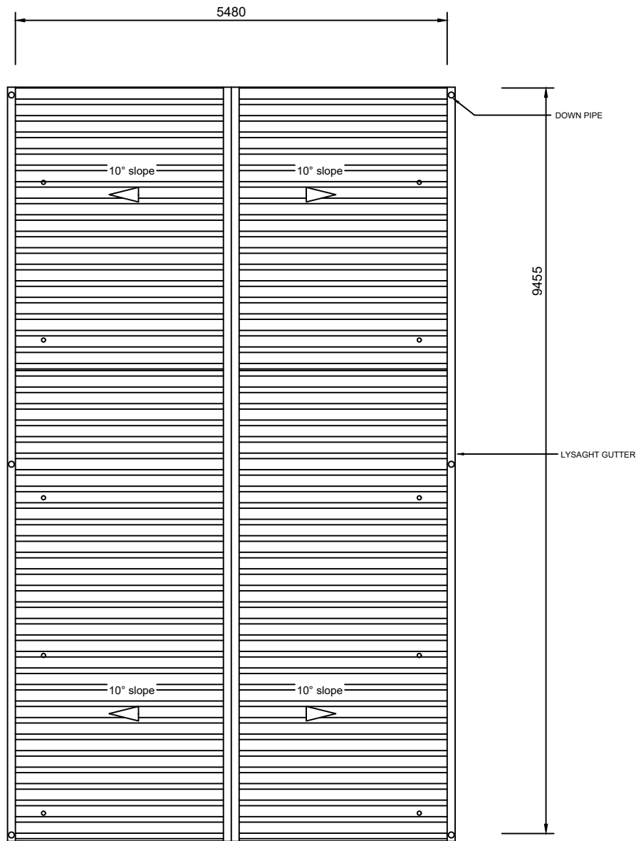
ROOF PLAN OVER WATER TANKS COUNCIL SITE
