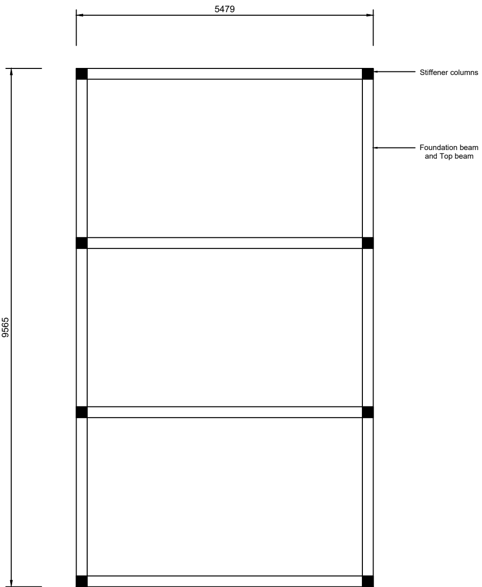
FOUNDATION PLAN COUNCIL SITE
