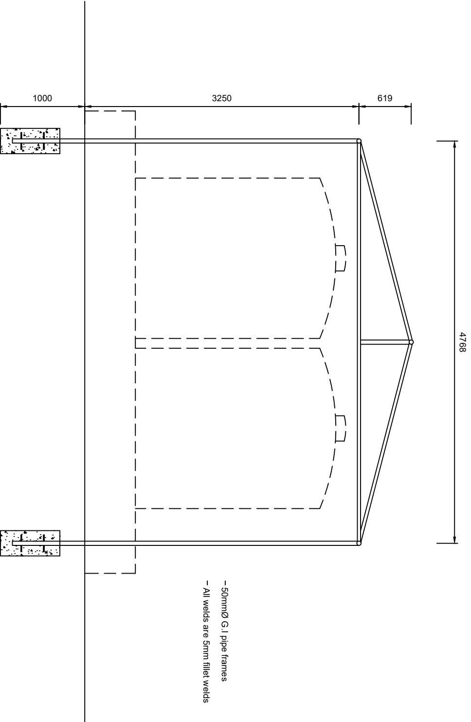
ROOF SUPPORTING FRAME DETAIL STAGE SITE
