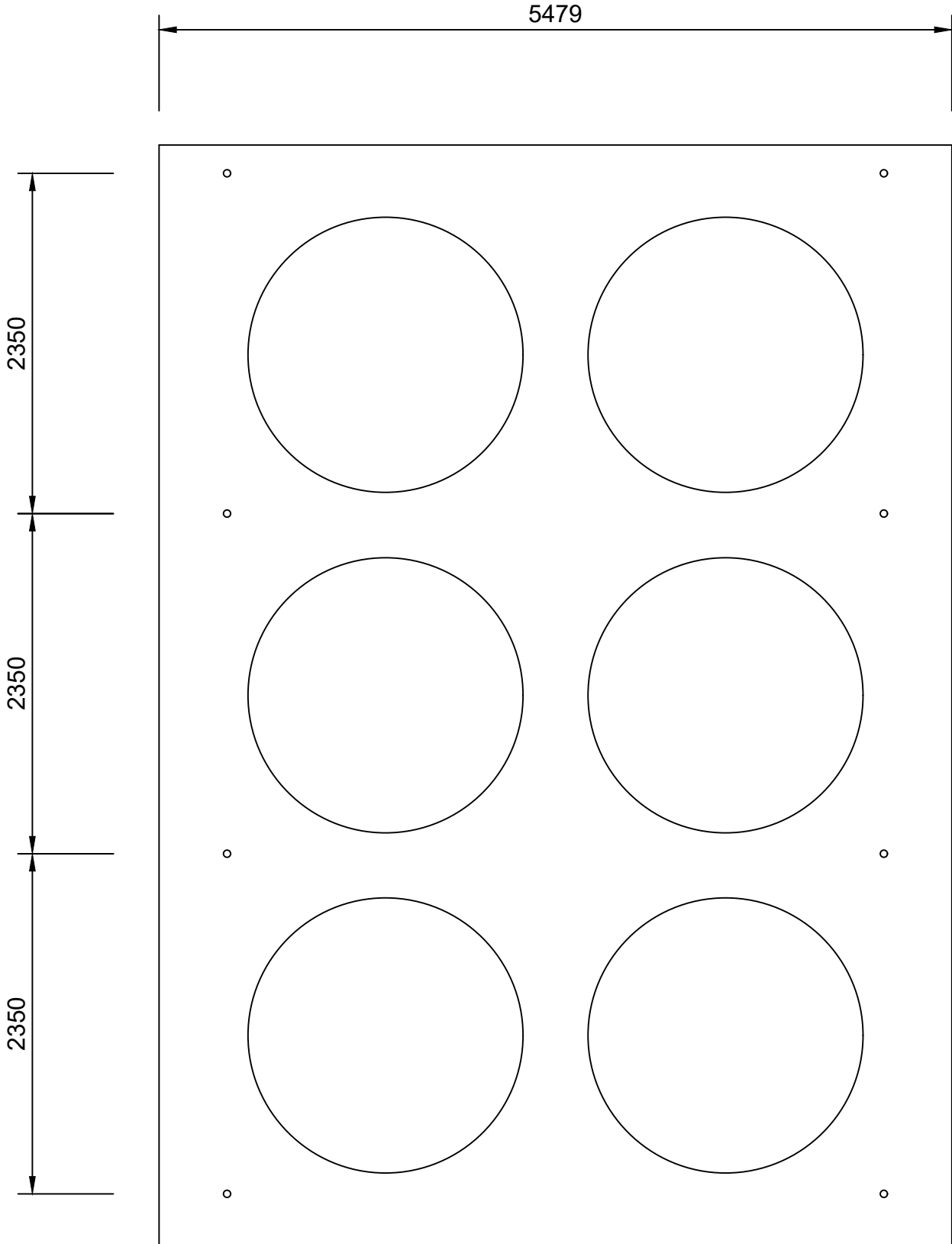
ROOF SUPPORTING PIPE ARRANGEMENT - PLAN STAGE SITE
