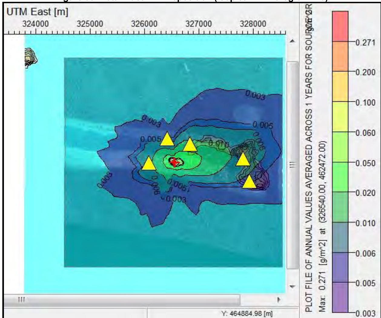
Figure 99: Total Dust 1YR Deposition (Isopleth in microgram/m 3 )
